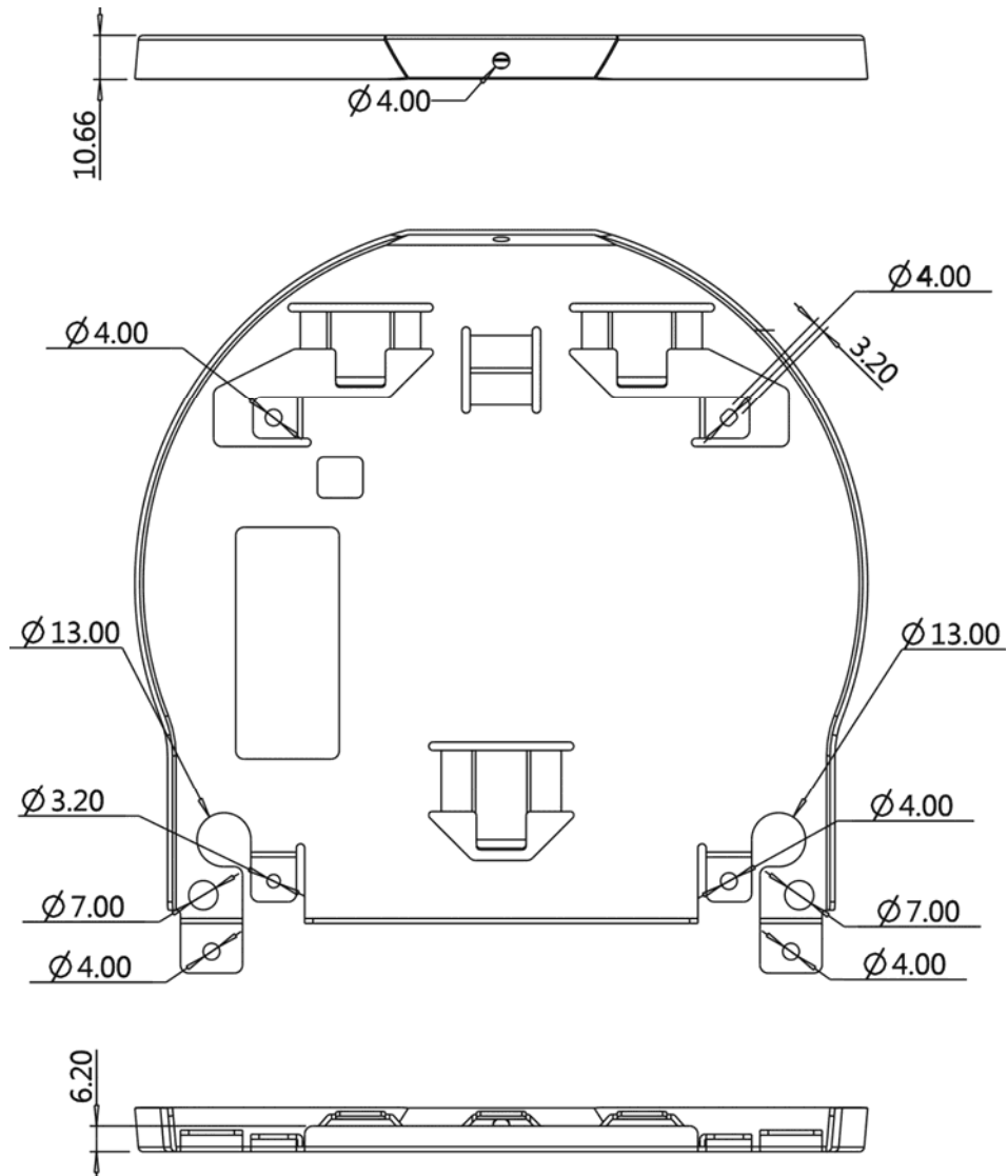
Metal plate A - machine side
